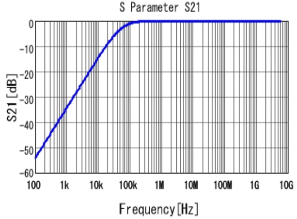
■ GCM155R71H333KE02 S21 DC0V, 25degC
