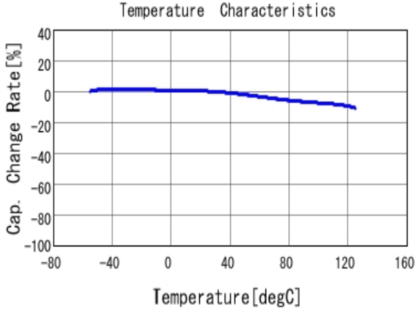
■ GCM155R71H333KE02 C-Temp. capchange, DC0.0V, AC1.0V r m
