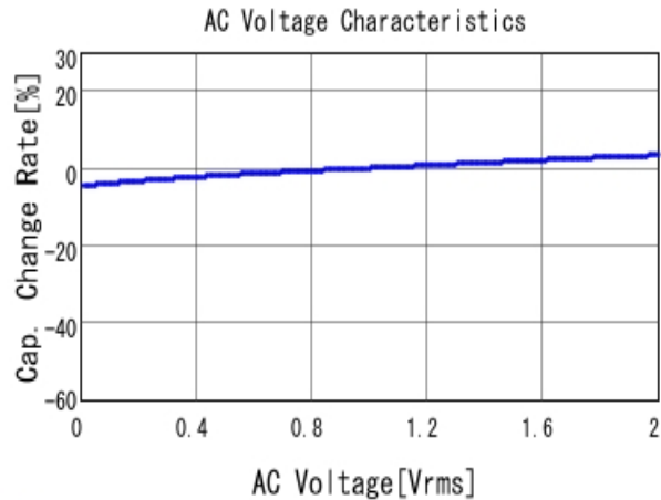
GCM155R71H333KE02 C-AC Voltage capchange, DCOV, 25.0d
