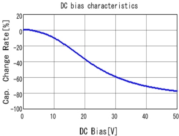
GCM155R71H333KE02 C-DC bias capchange, 25.0degC, AC1.
