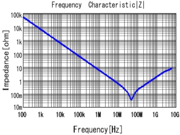
GCM155R71H333KE02 |Z| DCOV, 25degC
