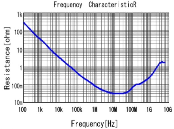
GCM155R71H333KE02 R DCOV, 25degC
