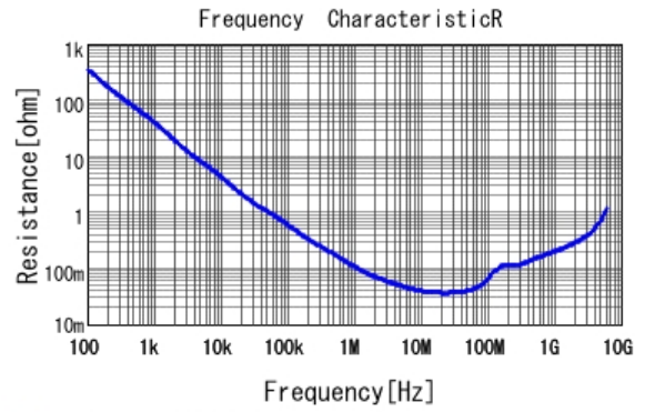
■ GCM155R71H223KA55 R DCOV, 25degC
