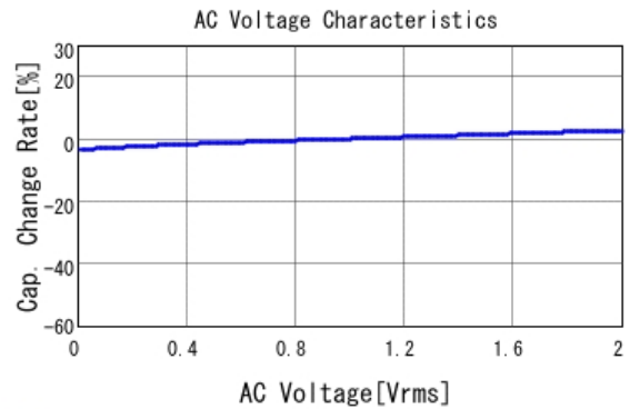
■ GCM155R71H223KA55 C-AC Voltage capchange, DCOV, 25.0d
