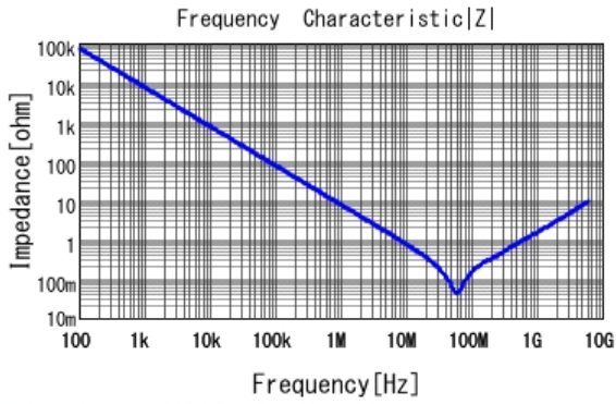
■ GCM155R71H223KA55 |Z| DCOV, 25degC
