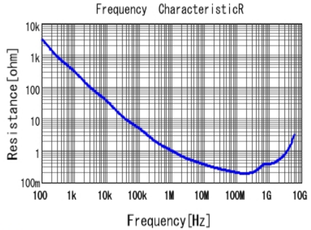
GCM155R71H222KA37 R DCOV, 25degC
