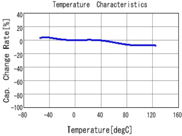
■ GCM155R71H222KA37 C-Temp. capchange, DCO. 0V, AC1.0Vrm
