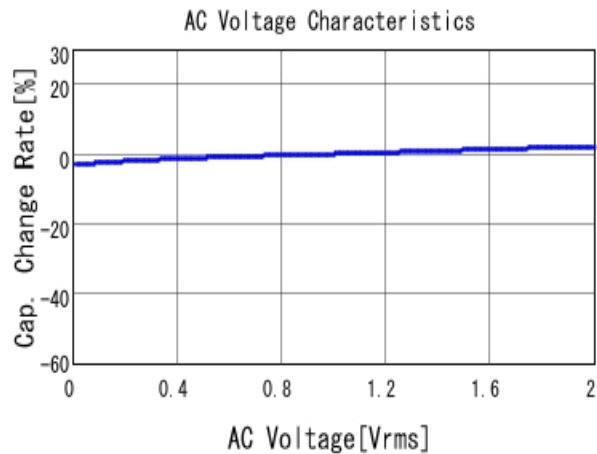
GCM155R71H222KA37 C-AC Voltage capchange, DCOV, 25.0d
