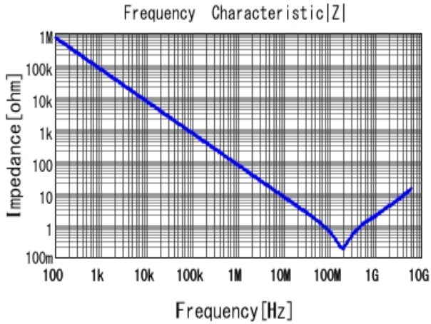
GCM155R71H222KA37 |Z| DCOV, 25degC
