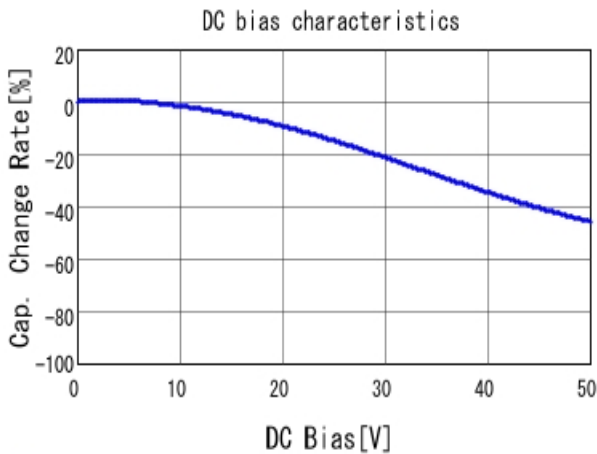
GCM155R71H222KA37 C-DC bias capchange, 25.0degC, AC1.
