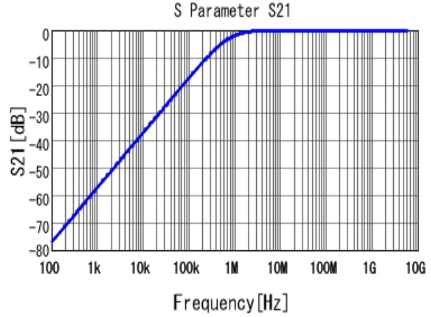
■ GCM155R71H222KA37 S21 DCOV, 25degC
