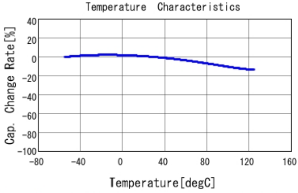
GCM155R71H104KE02 C-Temp. capchange, DC0.0V, AC1.C
