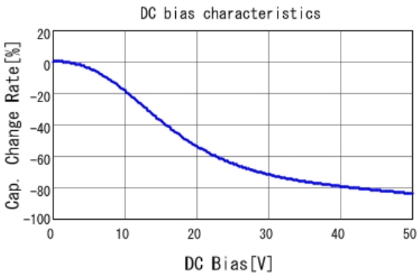
GCM155R71H104KE02 C-DC bias capchange, 25.0degC, A
