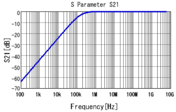
■ GCM155R71H103KA55 S21 DCOV, 25degC
