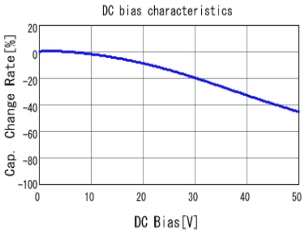
GCM155R71H103KA55 C-DC bias capchange, 25.0degC, AC1.
