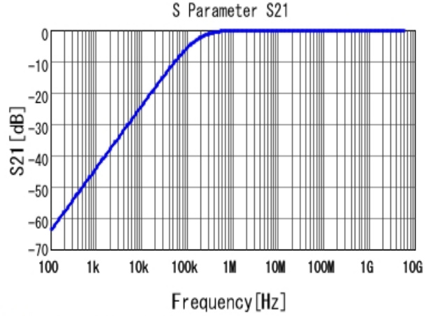
■ GCM155R71H103KA55 S21 DCOV, 25degC
