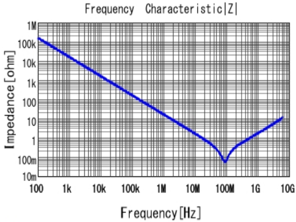
GCM155R71H103KA55 |Z| DC0V, 25degC
