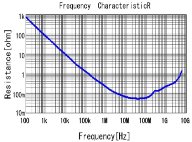
GCM155R71H103KA55 R DC0V, 25degC
