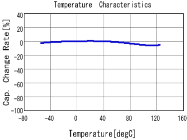
■ GCM155R71H103KA55 C-Temp. capchange, DCO. 0V, AC1.0Vrm
