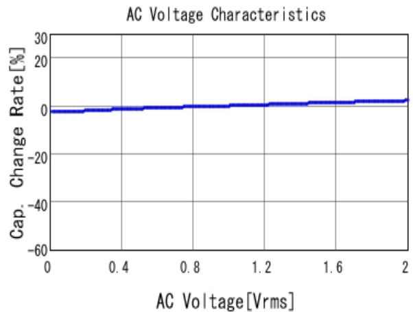
GCM155R71H103KA55 C-AC Voltage capchange, DC0V, 25.0d
