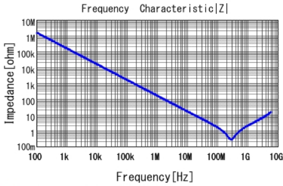
GCM155R71H102KA37 |Z| DCOV, 25degC
