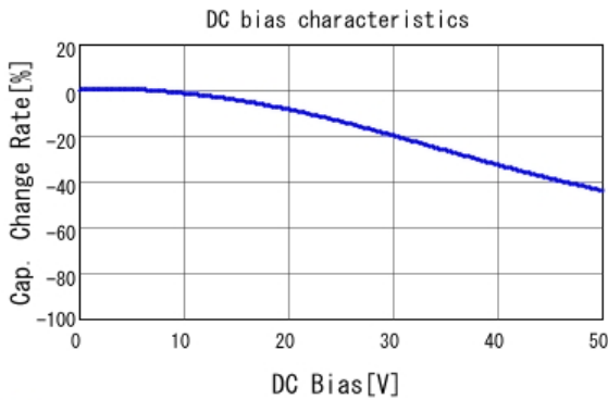
GCM155R71H102KA37 C-DC bias capchange, 25.0degC, AC1.
