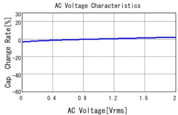
GCM155R71H102KA37 C-AC Voltage capchange, DCOV, 25.0d
