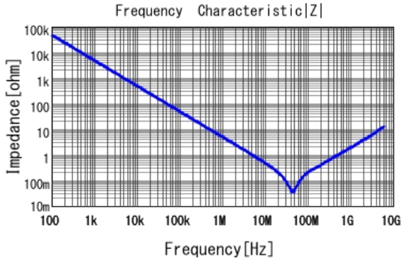
GCM155R71E333KA55 |Z| DCOV, 25degC
