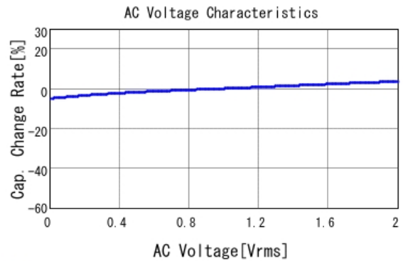
GCM155R71E333KA55 C-AC Voltage capchange, DCOV, 25.0d
