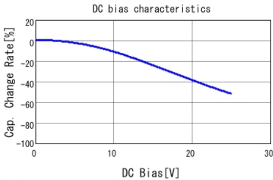
GCM155R71E333KA55 C-DC bias capchange, 25.0degC, AC1.
