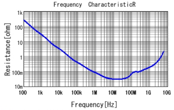
GCM155R71E333KA55 R DCOV, 25degC
