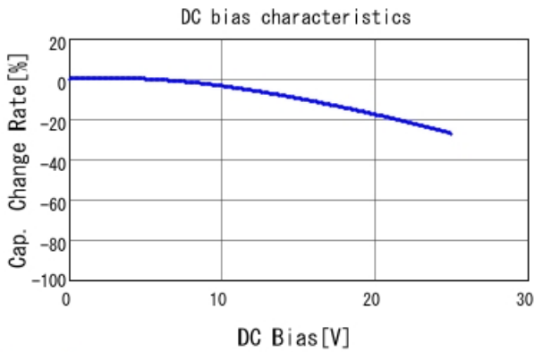
GCM155R71E103KA37 C-DC bias capchange, 25.0degC, A
