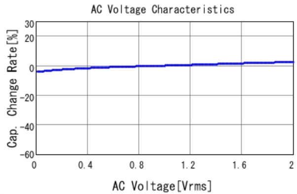
GCM155R71E103KA37 C-AC Voltage capchange, DCOV, 25
