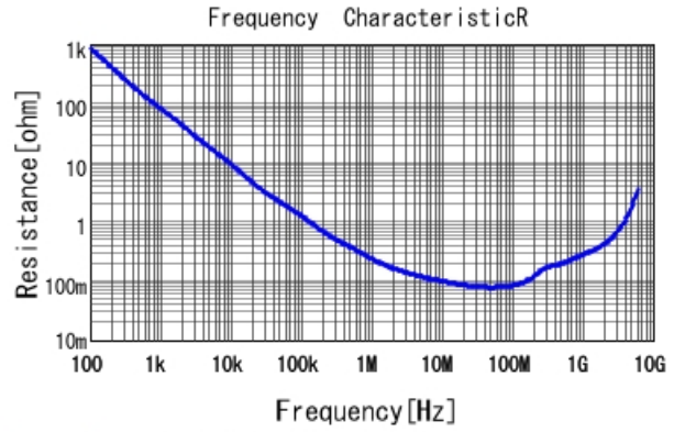
GCM155R71E103KA37 R DCOV, 25degC
