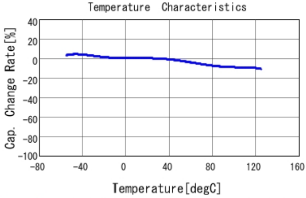
GCM155R71E103KA37 C-Temp. capchange, DC0.0V, AC1.C
