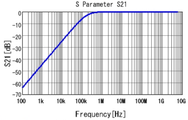
GCM155R71E103KA37 S21 DC0V, 25degC
