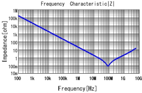
GCM155R71E103KA37 |Z| DCOV, 25degC
