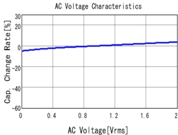
GCM155R71C333KA37 C-AC Voltage capchange, DCOV, 25.0d
