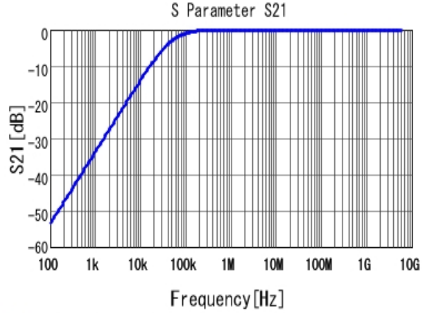
■ GCM155R71C333KA37 S21 DC0V, 25degC
