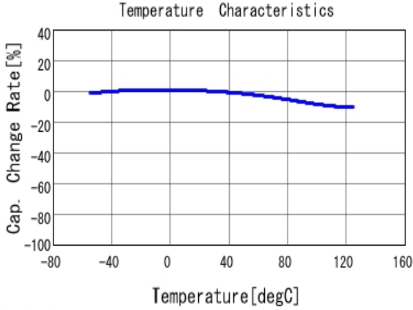
■ GCM155R71C333KA37 C-Temp. capchange, DC0.0V, AC1.0V rm
