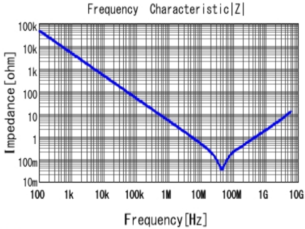
GCM155R71C333KA37 |Z| DCOV, 25degC
