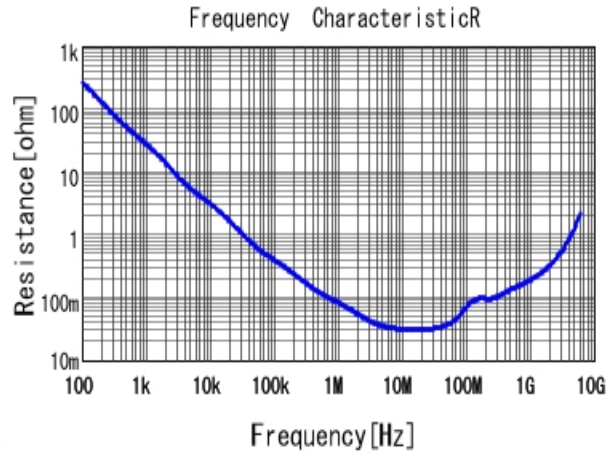
GCM155R71C333KA37 R DCOV, 25degC
