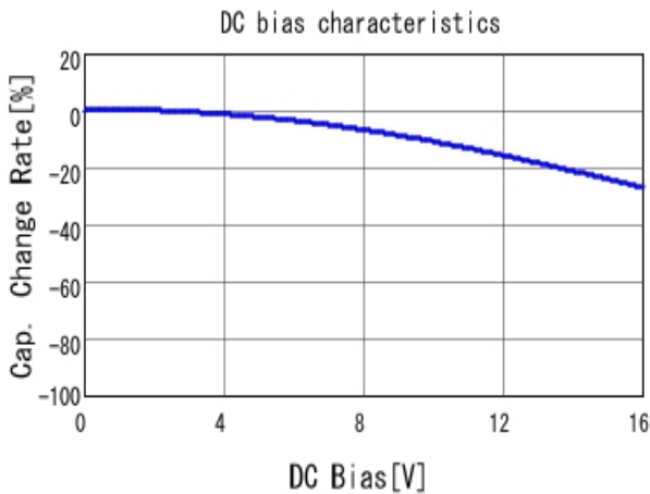
GCM155R71C333KA37 C-DC bias capchange, 25.0degC, AC1.
