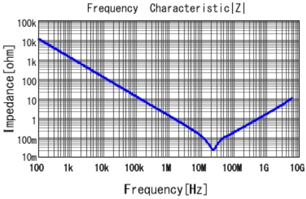
GCM155R71C224KE02 |Z| DCOV, 25degC
