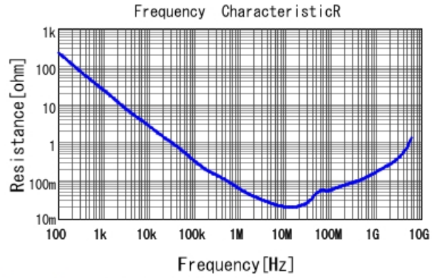
GCM155R71C224KE02 R DCOV, 25degC
