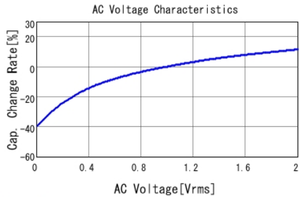
GCM155R71C224KE02 C-AC Voltage capchange, DCOV, 25
