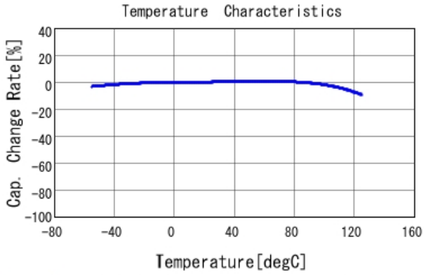
GCM155R71C224KE02 C-Temp. capchange, DC0.0V, AC1.C
