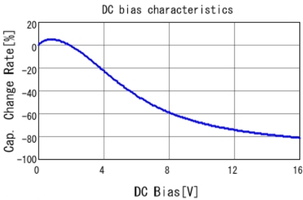
GCM155R71C224KE02 C-DC bias capchange, 25.0degC, A
