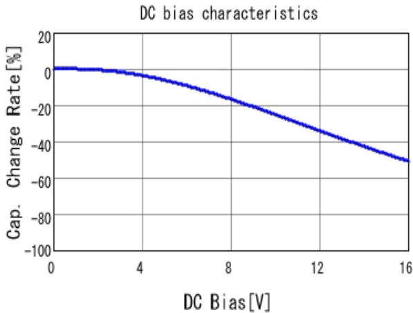
GCM155R71C104KA55 C-DC bias capchange, 25.0degC, AC1.
