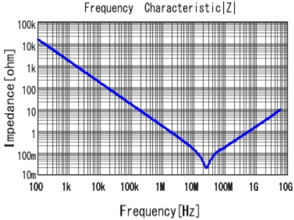
GCM155R71C104KA55 |Z| DCOV, 25degC
