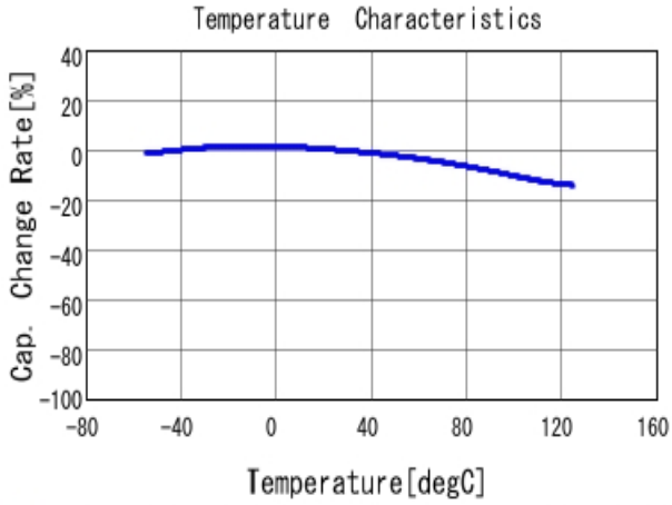
GCM155R71C104KA55 C-Temp. capchange, DC0.0V, AC1.0V rm
