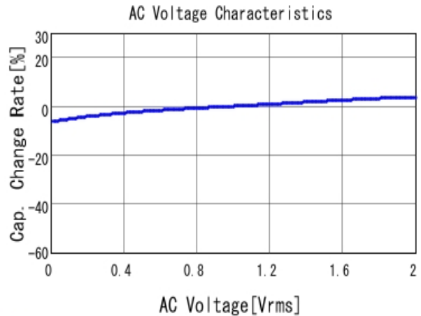
GCM155R71C104KA55 C-AC Voltage capchange, DCOV, 25.0d
