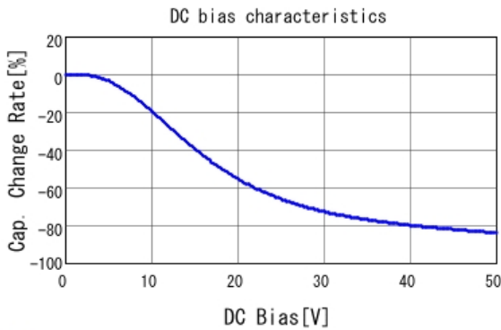
GCM155L8EH104KE07 C-DC bias capchange, 25.0degC, AC1.
