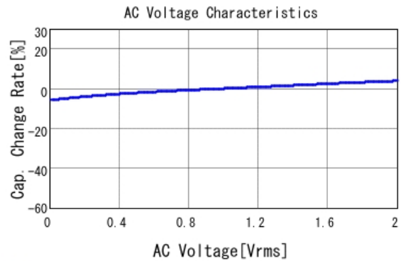
GCM155L8EH104KE07 C-AC Voltage capchange, DC0V, 25.0d
