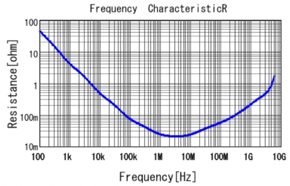
GCM155C71A684KE38 R DC0V, 25degC
