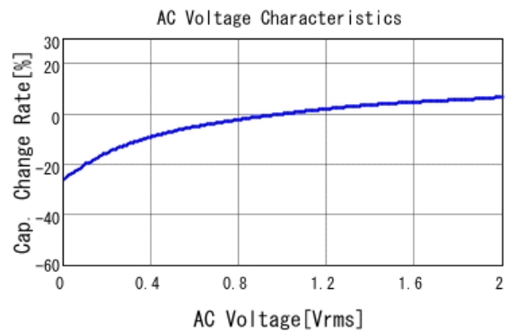
GCM155C71A684KE38 C-AC Voltage capchange, DC0V, 25.0d
