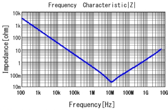
GCM155C71A684KE38 |Z| DC0V, 25degC
