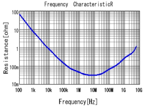
GCM155C71A474KE36 R DCOV, 25degC
