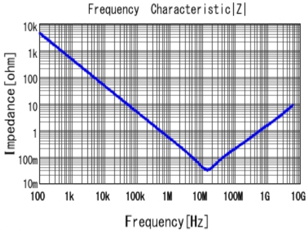
GCM155C71A474KE36 |Z| DCOV, 25degC
