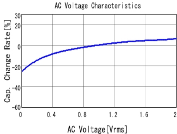
GCM155C71A474KE36 C-AC Voltage capchange, DCOV, 25.0d
