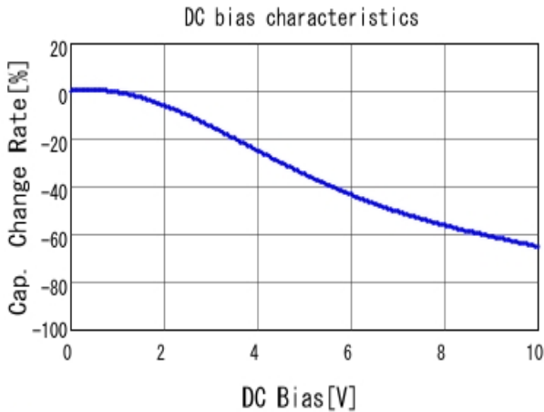
GCM155C71A474KE36 C-DC bias capchange, 25.0degC, AC1V
