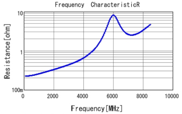
GCM1555C1H8R0BA16 R DCOV, 25degC
