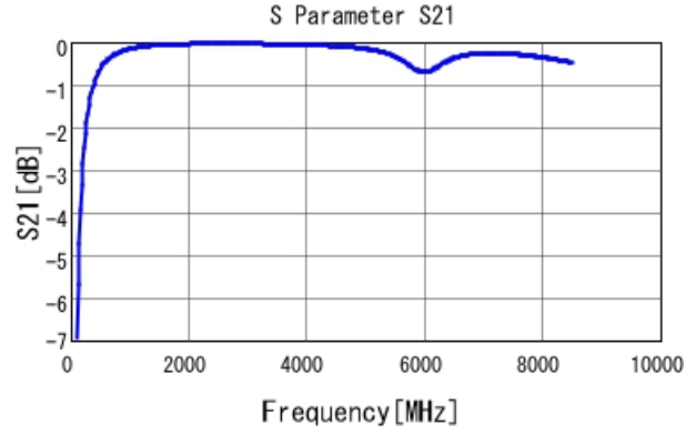
GCM1555C1H8R0BA16 S21 DCOV, 25degC
