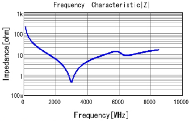
GCM1555C1H8R0BA16 |Z| DCOV, 25degC
