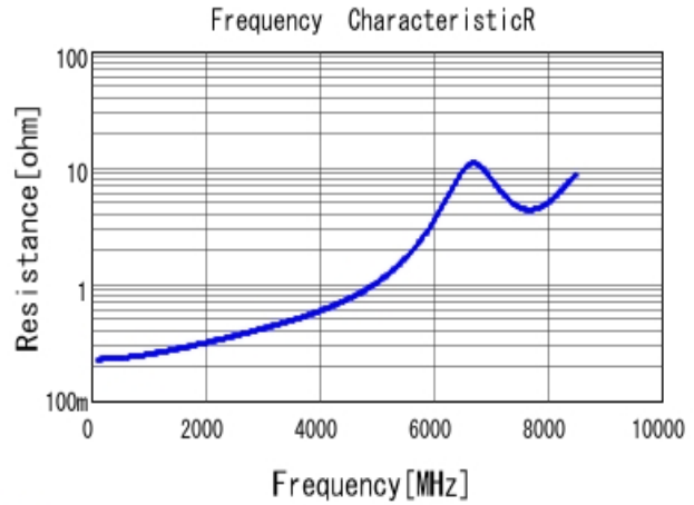
■ GCM1555C1H6R8CA16 R DCOV, 25degC
