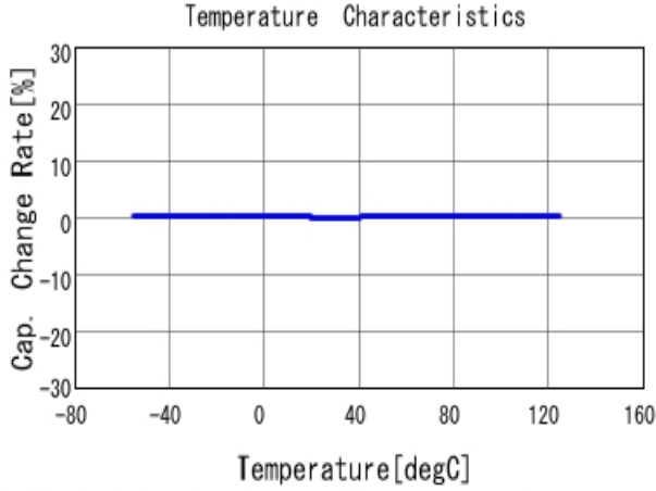
■ GCM1555C1H6R8CA16 C-Temp. capchange, DCOV, AC1Vrms
