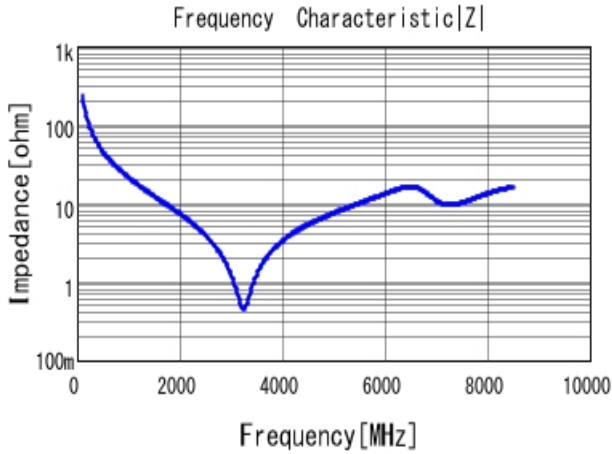
■ GCM1555C1H6R8CA16 |Z| DCOV, 25degC
