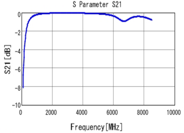
■ GCM1555C1H6R8CA16 S21 DCOV, 25degC
