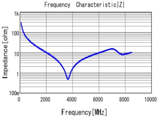
GCM1555C1H5R6DA16 |Z| DC0V, 25degC
