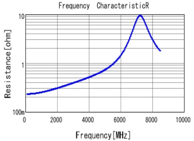
GCM1555C1H5R6DA16 R DC0V, 25degC
