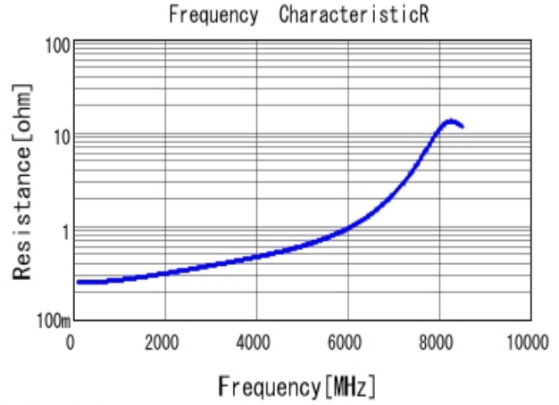
GCM1555C1H4R3BA16 R DC0V, 25degC
