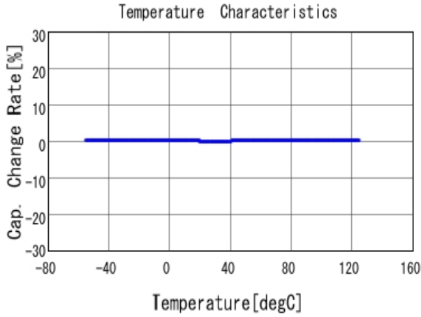
■ GCM1555C1H4R3BA16 C-Temp. capchange, DCOV, AC1Vrms
