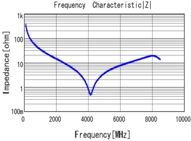
GCM1555C1H4R3BA16 |Z| DC0V, 25degC
