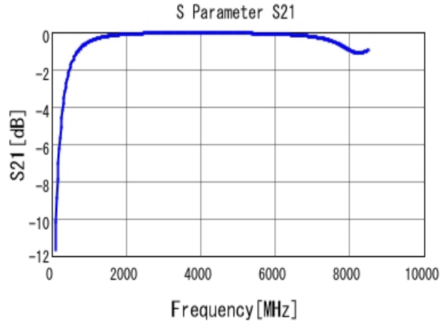
■ GCM1555C1H4R3BA16 S21 DCOV, 25degC
