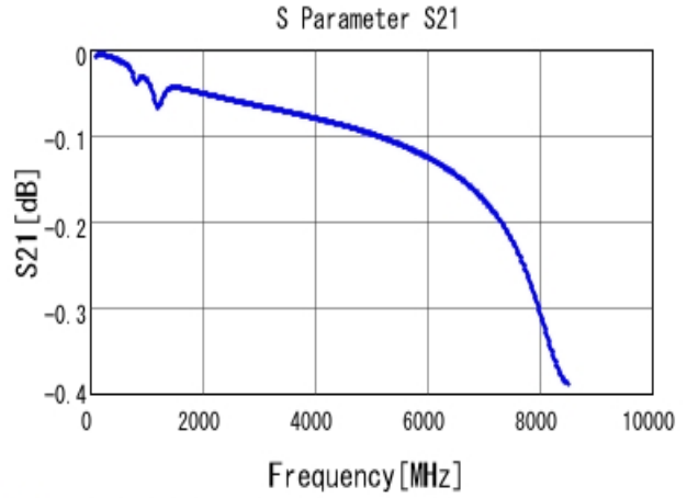
■ GCM1555C1H471JA16 S21 DCOV, 25degC
