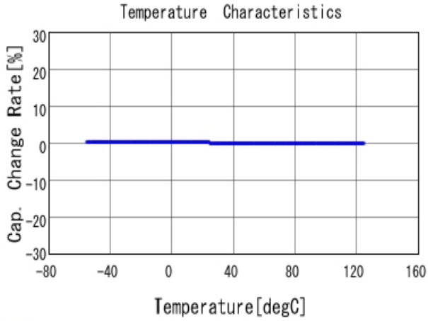
■ GCM1555C1H471JA16 C-Temp. capchange, DCOV, AC1Vrms
