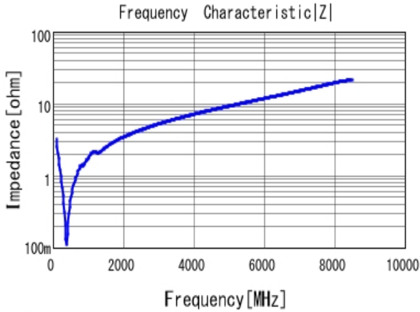
GCM1555C1H471JA16 |Z| DC0V, 25degC
