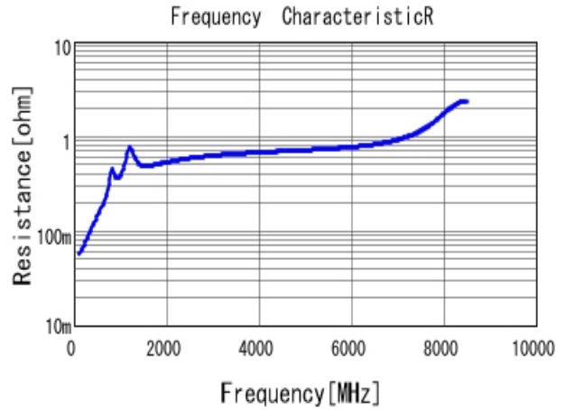
GCM1555C1H471JA16 R DC0V, 25degC
