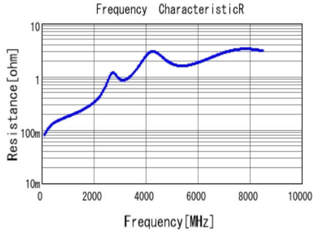
GCM1555C1H470JA16 R DC0V, 25degC
