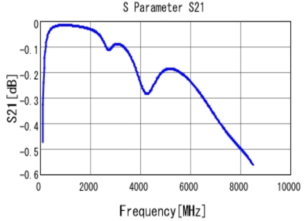
■ GCM1555C1H470JA16 S21 DCOV, 25degC
