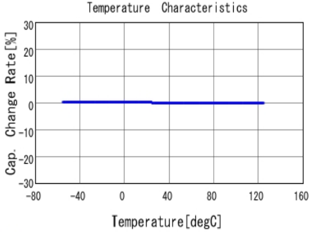
■ GCM1555C1H470JA16 C-Temp. capchange, DCOV, AC1Vrms
