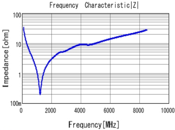
GCM1555C1H470JA16 |Z| DC0V, 25degC
