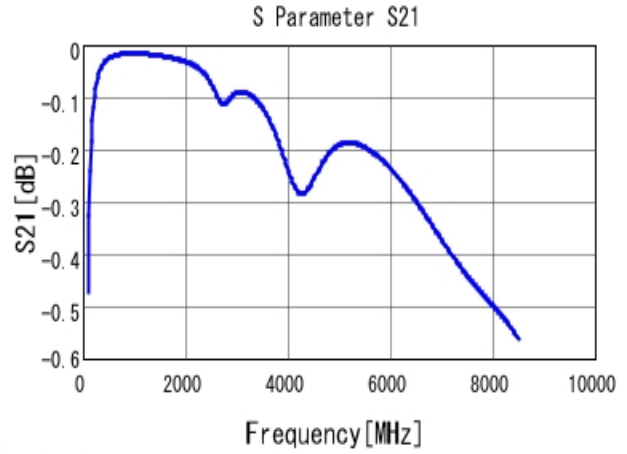
■ GCM1555C1H470JA16 S21 DCOV, 25degC
