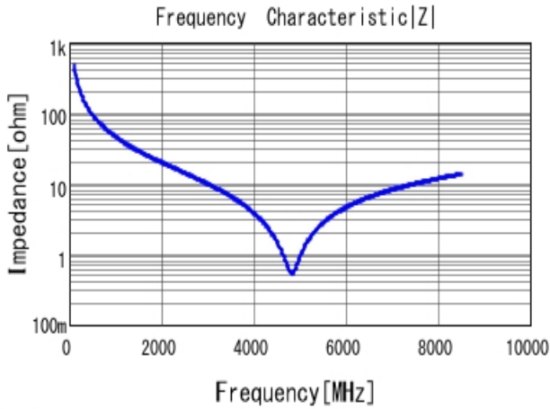
GCM1555C1H3R3CA16 |Z| DCOV, 25degC
