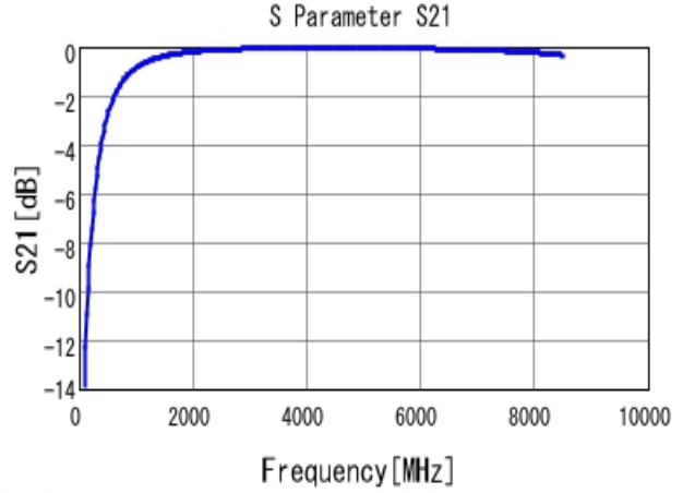
■ GCM1555C1H3R3CA16 S21 DCOV, 25degC
