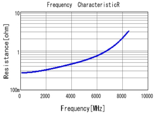
GCM1555C1H3R3CA16 R DCOV, 25degC
