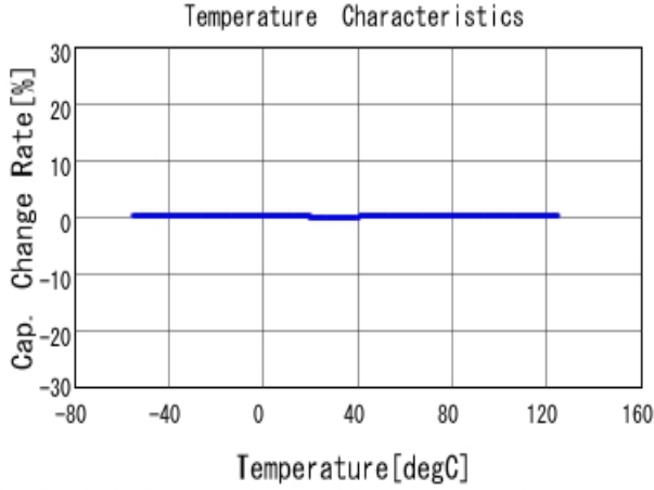
■ GCM1555C1H3R3CA16 C-Temp. capchange, DCOV, AC1Vrms
