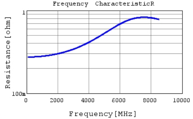
GCM1555C1H3R0BA16 R DCOV, 25degC
