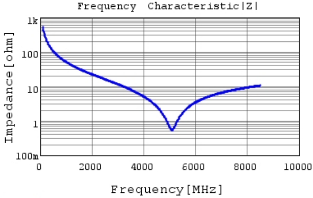
GCM1555C1H3R0BA16 |Z| DCOV, 25degC
