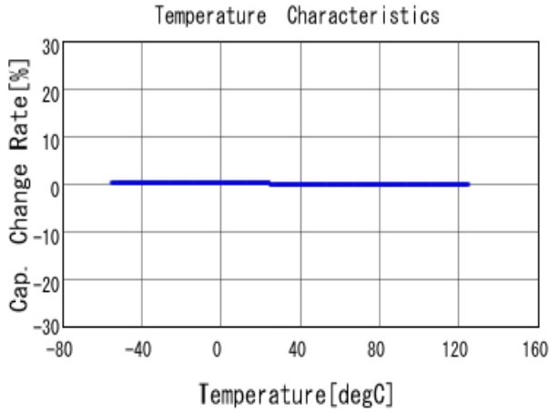
■ GCM1555C1H391JA16 C-Temp. capchange, DCOV, AC1Vrms
