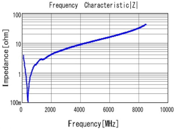
■ GCM1555C1H391JA16 |Z| DC0V, 25degC
