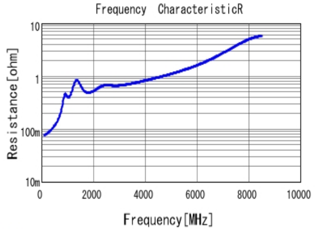
■ GCM1555C1H391JA16 R DC0V, 25degC
