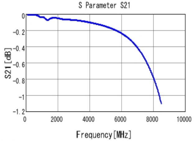
■ GCM1555C1H391JA16 S21 DCOV, 25degC
