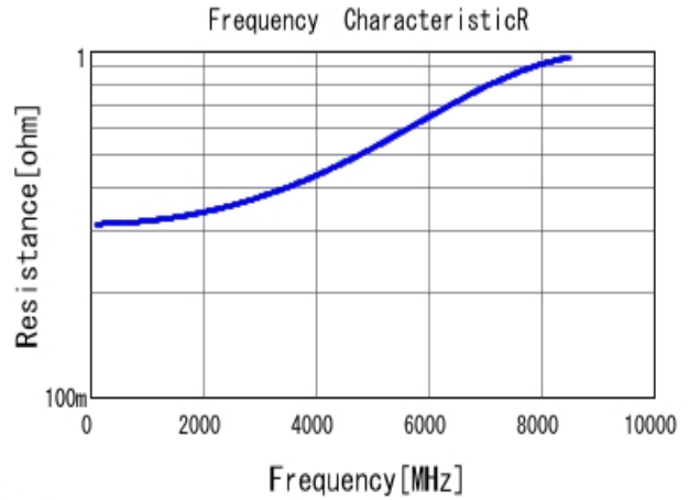
GCM1555C1H2R2CA16 R DC0V, 25degC
