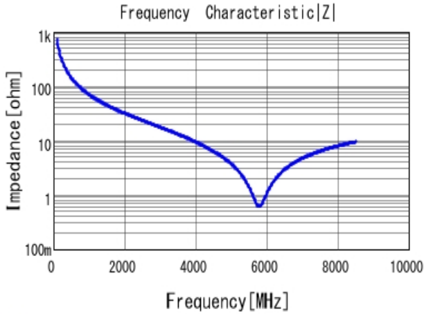
GCM1555C1H2R2CA16 |Z| DC0V, 25degC
