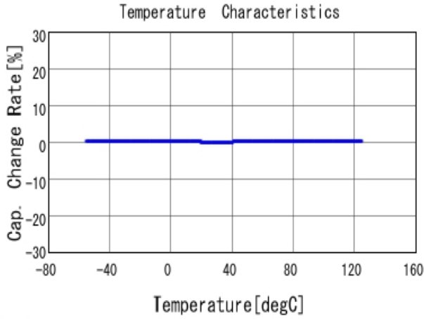
■ GCM1555C1H2R2CA16 C-Temp. capchange, DCOV, AC1Vrms
