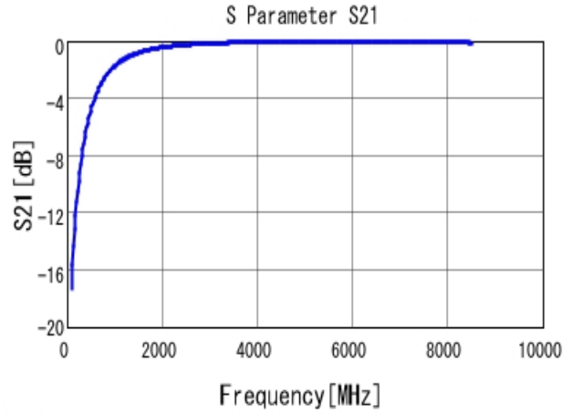
■ GCM1555C1H2R2CA16 S21 DCOV, 25degC
