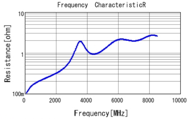
■ GCM1555C1H270JA16 R DC0V, 25degC
