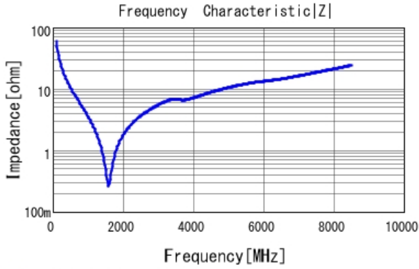
■ GCM1555C1H270JA16 |Z| DC0V, 25degC
