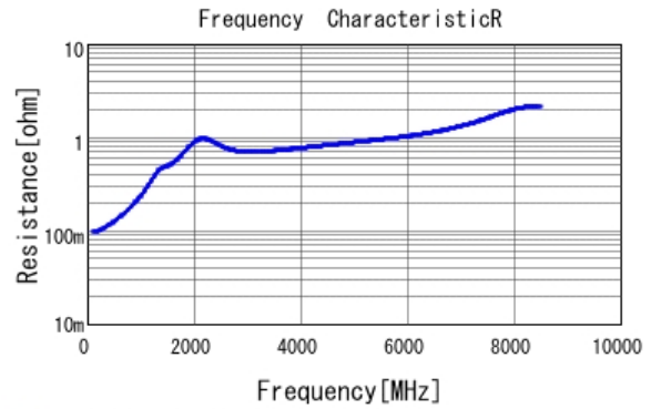
■ GCM1555C1H221JA16 R DC0V, 25degC
