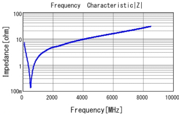
■ GCM1555C1H221JA16 |Z| DC0V, 25degC
