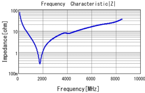
■ GCM1555C1H220JA16 |Z| DC0V, 25degC
