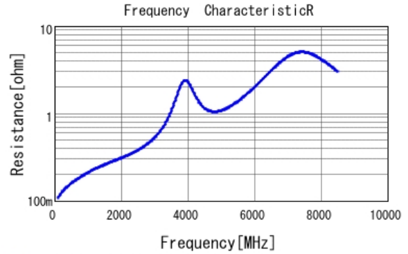
■ GCM1555C1H220JA16 R DC0V, 25degC
