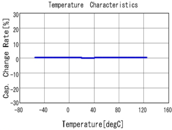
■ GCM1555C1H1R8CA16 C-Temp. capchange, DCOV, AC1Vrms
