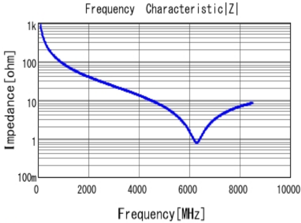
■ GCM1555C1H1R8CA16 |Z| DC0V, 25degC
