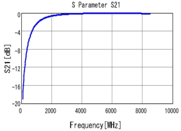
■ GCM1555C1H1R8CA16 S21 DCOV, 25degC
