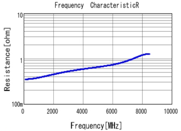
■ GCM1555C1H1R8CA16 R DC0V, 25degC
