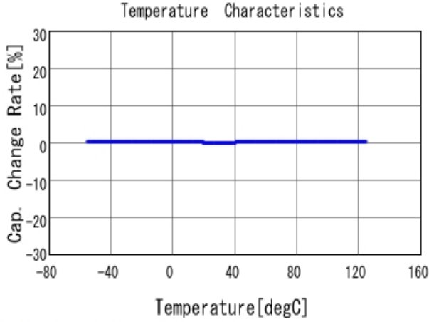
■ GCM1555C1H1R5JA16 C-Temp. capchange, DCOV, AC1Vrms
