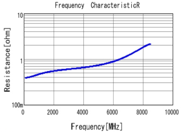
GCM1555C1H1R5JA16 R DCOV, 25degC
