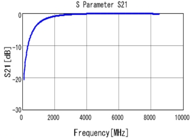
■ GCM1555C1H1R5JA16 S21 DCOV, 25degC
