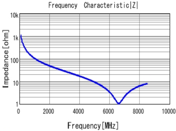
GCM1555C1H1R5JA16 |Z| DCOV, 25degC
