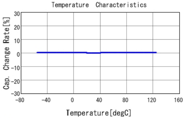
■ GCM1555C1H1R0JA16 C-Temp. capchange, DCOV, AC1Vrms
