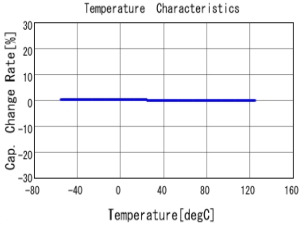
■ GCM1555C1H150JA16 C-Temp. capchange, DCOV, AC1Vrms
