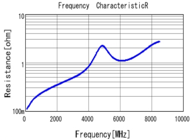
■ GCM1555C1H150JA16 R DC0V, 25degC
