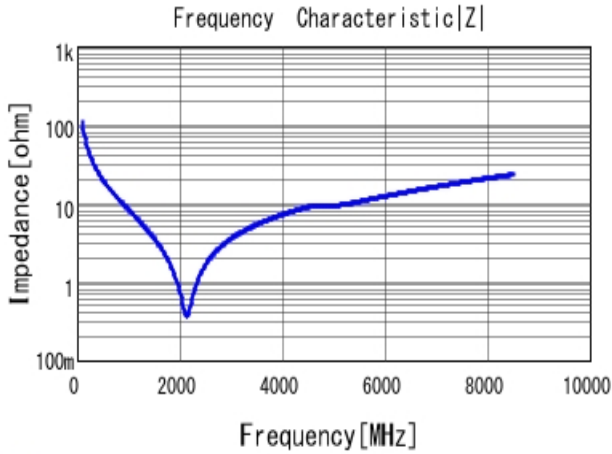
■ GCM1555C1H150JA16 |Z| DC0V, 25degC
