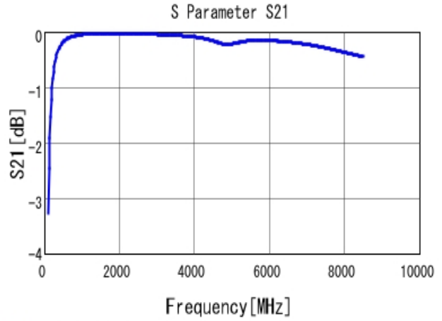
■ GCM1555C1H150JA16 S21 DCOV, 25degC
