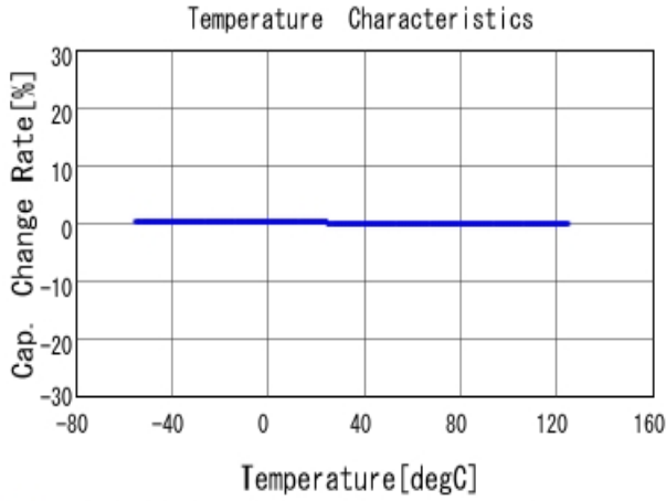
■ GCM1555C1H120JA16 C-Temp. capchange, DCOV, AC1Vrms
