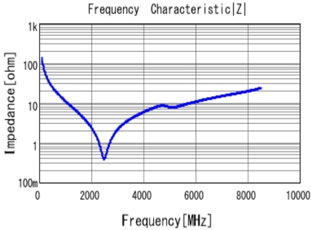
■ GCM1555C1H120JA16 |Z| DC0V, 25degC
