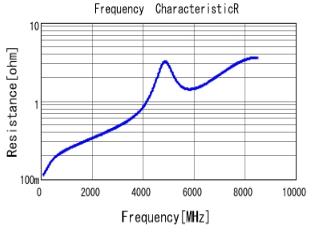
■ GCM1555C1H120JA16 R DC0V, 25degC
