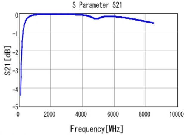
■ GCM1555C1H120JA16 S21 DCOV, 25degC
