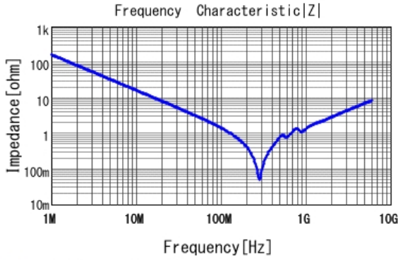
GCM1555C1H102JA16 |Z| DCOV, 25degC
