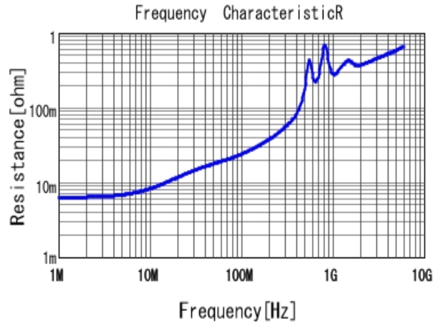
GCM1555C1H102JA16 R DCOV, 25degC
