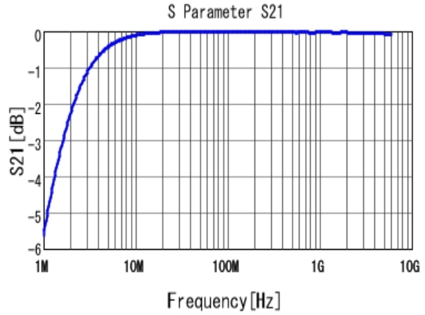
■ GCM1555C1H102JA16 S21 DCOV, 25degC
