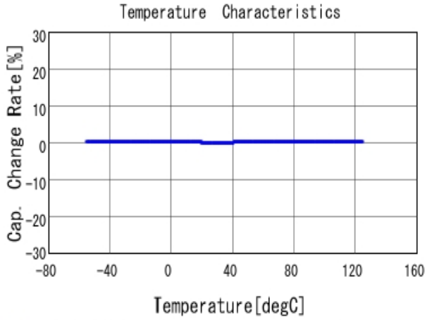
■ GCM1555C1H102JA16 C-Temp. capchange, DCOV, AC1Vrms
