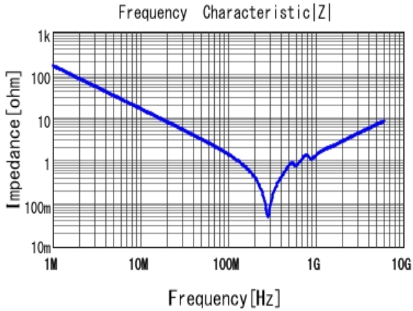
GCM1555C1H102JA16 |Z| DCOV, 25degC
