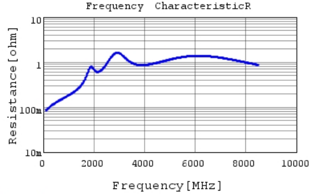
GCM1555C1H101JA16 R DCOV,25degC
