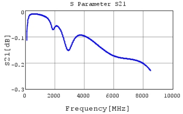
GCM1555C1H101JA16 S21 DCOV, 25degC
