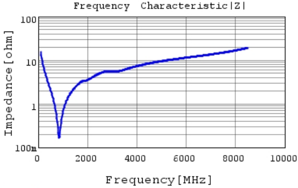
GCM1555C1H101JA16 |Z| DCOV,25degC
