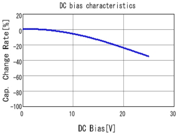
GCM033R71E102KA03 C-DC bias capchange, 25.0degC, AC1.
