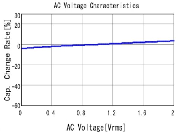
GCM033R71E102KA03 C-AC Voltage capchange, DC0V, 25.0d
