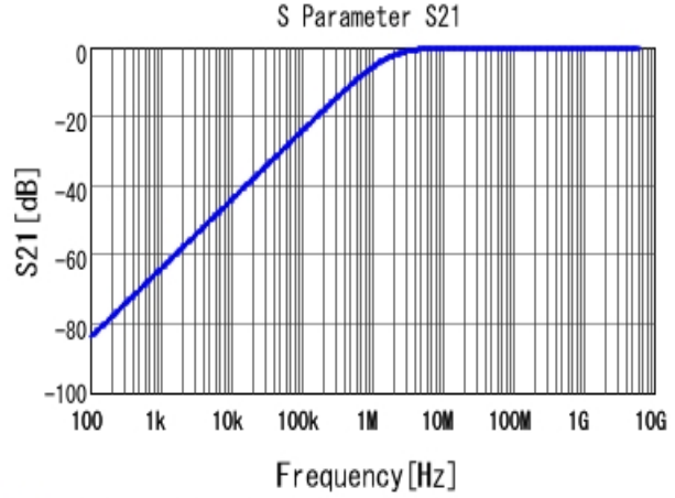
■ GCM033R71E102KA03 S21 DC0V, 25degC
