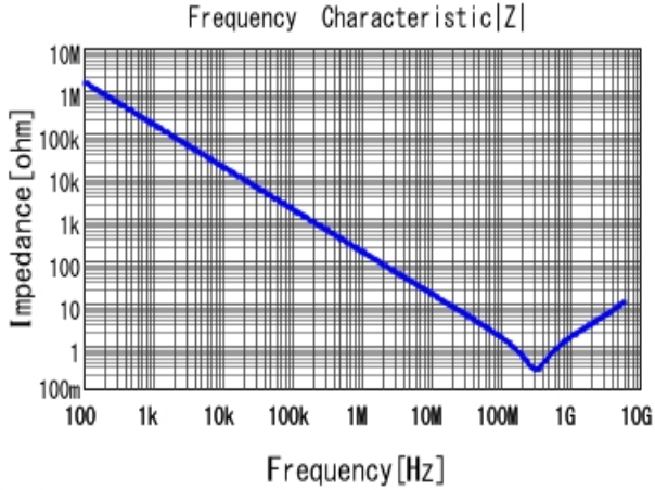
GCM033R71E102KA03 |Z| DC0V, 25degC
