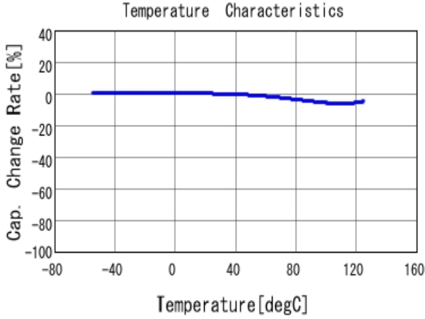
■ GCM033R71E102KA03 C-Temp. capchange, DC0.0V, AC1.0V rm
