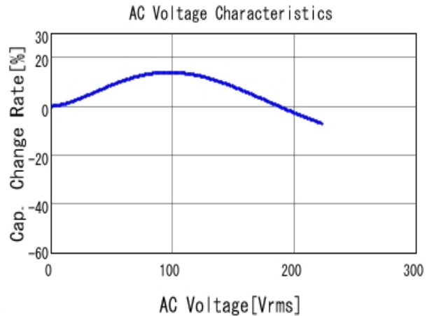
■ GCJ43DR72J104KXJ1 C-AC Voltage capchange, DC0V, 25.0d
