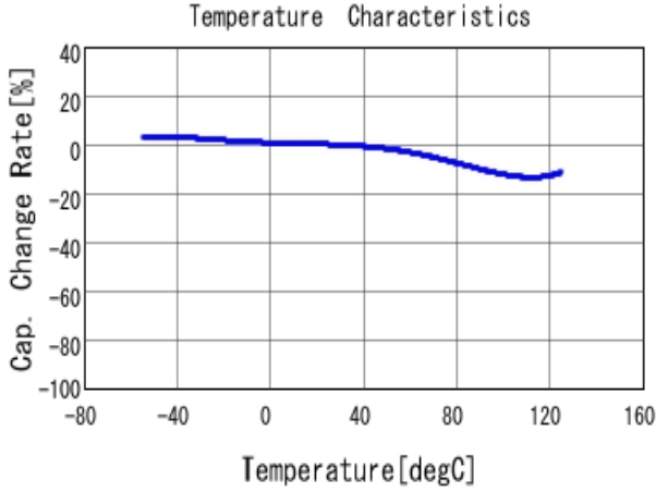
GCJ43DR72J104KXJ1 C-Temp. capchange, DCOV, AC1Vrms
