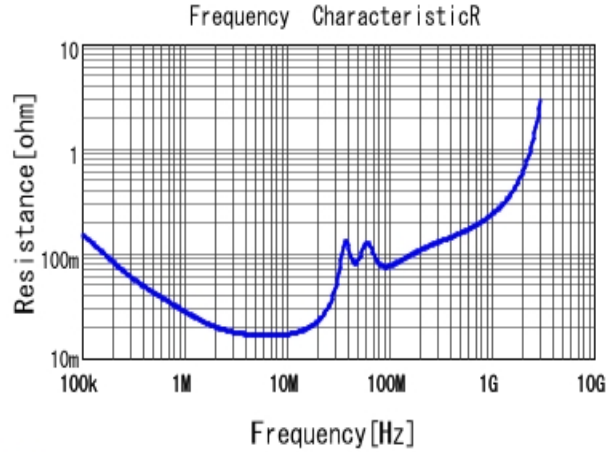
■ GCJ43DR72J104KXJ1 R DC0V, 25degC
