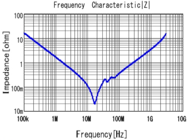
■ GCJ43DR72J104KXJ1 |Z| DC0V, 25degC
