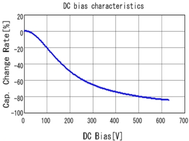
■ GCJ43DR72J104KXJ1 C-DC bias capchange, 25.0degC, AC1V
