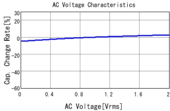
■ GCJ32EC71H106KA01 C-AC Voltage capchange, DC0V, 25.0d
