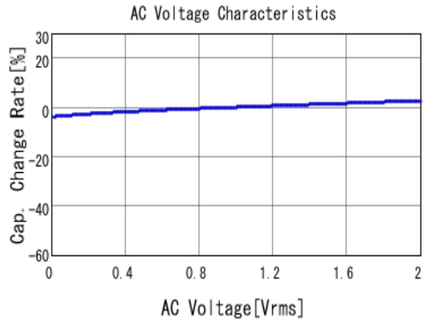
■ GCJ21BR72A104KA01 C-AC Voltage capchange, DCOV, 25.0d
