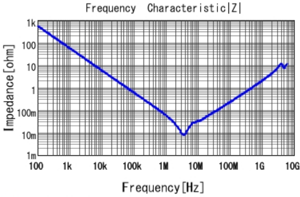
■ GCJ21BR71C475KA01 |Z| DC0V, 25degC
