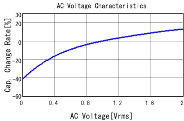
■ GCJ21BR71C475KA01 C-AC Voltage capchange, DC0V, 25.0d
