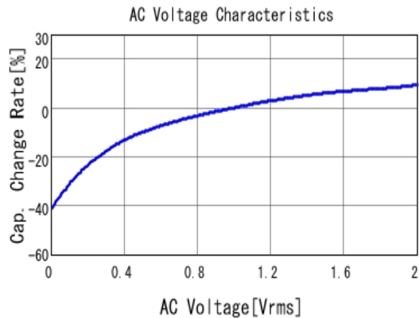
■ GCJ21BR71A106KE01 C-AC Voltage capchange, DCOV, 25.0d
