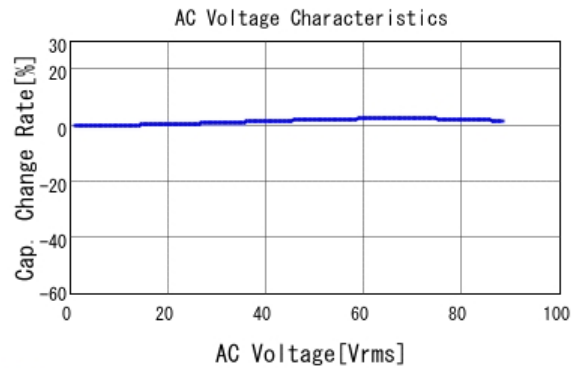
■ GCJ21AR72E472KXJ1 C-AC Voltage capchange, DC0V, 25.0d
