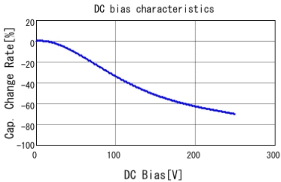
■ GCJ21AR72E472KXJ1 C-DC bias capchange, 25.0degC, AC1V
