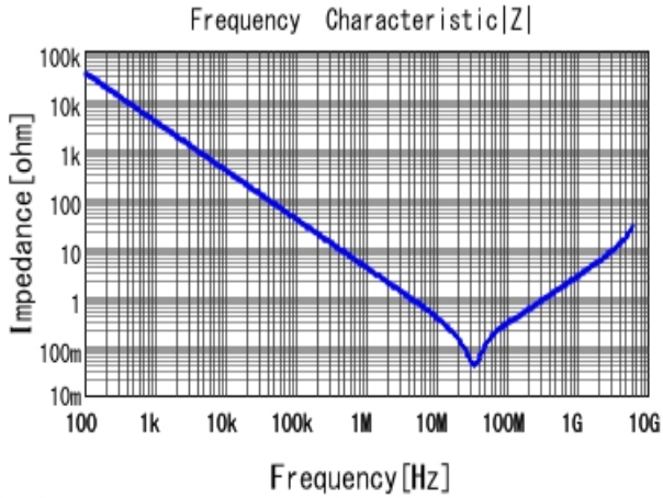
■ GCJ188R92A473KA01 |Z| DC0V, 25degC
