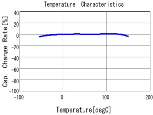
■ GCJ188R92A473KA01 C-Temp. capchange, DC0.0V, AC1.0V rm
