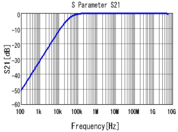
■ GCJ188R92A473KA01 S21 DC0V, 25degC
