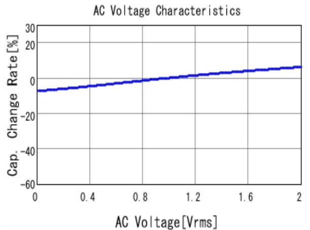
■ GCJ188R92A473KA01 C-AC Voltage capchange, DC0V, 25.0d
