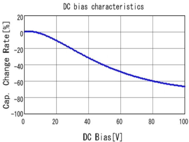
■ GCJ188R92A473KA01 C-DC bias capchange, 25.0degC, AC1.
