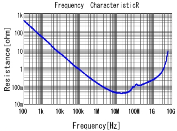
■ GCJ188R92A473KA01 R DC0V, 25degC
