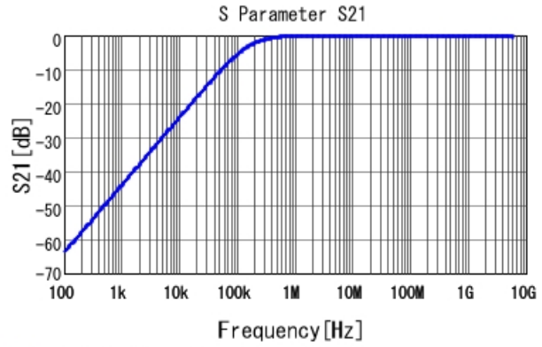
■ GCJ188R72A103KA01 S21 DCOV, 25degC
