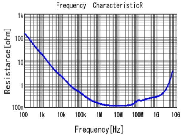
■ GCJ188R71H473KA12 R DCOV, 25degC
