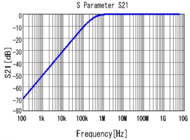
■ GCJ188R71H472KA01 S21 DCOV, 25degC
