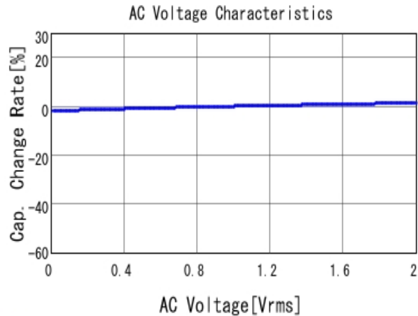
■ GCJ188R71H472KA01 C-AC Voltage capchange, DCOV, 25.0d
