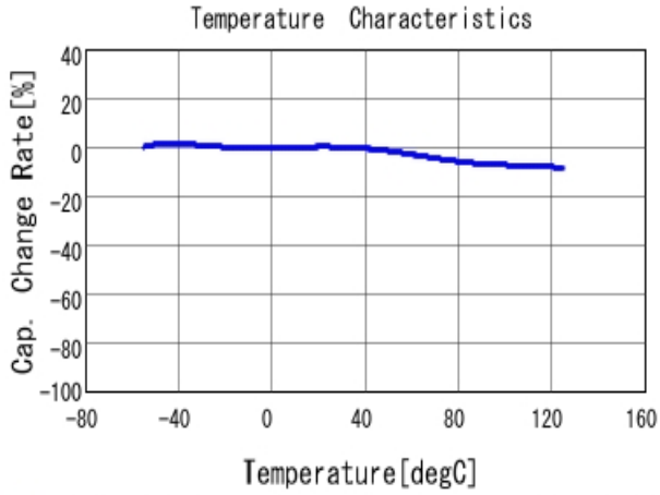
■ GCJ188R71H472KA01 C-Temp. capchange, DCO. 0V, AC1.0Vrm
