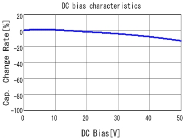
■ GCJ188R71H472KA01 C-DC bias capchange, 25.0degC, AC1.
