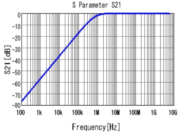
■ GCJ188R71H222KA01 S21 DCOV, 25degC
