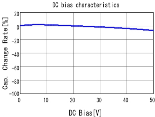
■ GCJ188R71H222KA01 C-DC bias capchange, 25.0degC, AC1.
