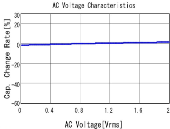
■ GCJ188R71H222KA01 C-AC Voltage capchange, DCOV, 25.0d
