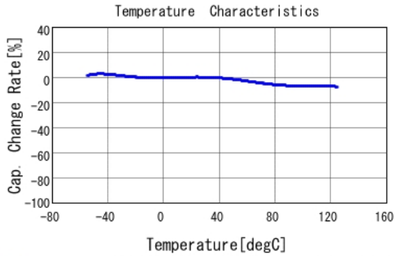
■ GCJ188R71H103KA01 C-Temp. capchange, DC0.0V, AC1.0Vrm
