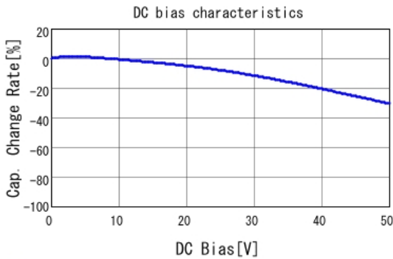
■ GCJ188R71H103KA01 C-DC bias capchange, 25.0degC, AC1.
