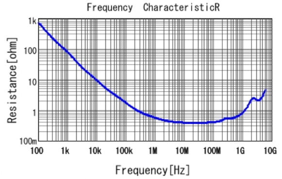
■ GCJ188R71H103KA01 R DCOV, 25degC
