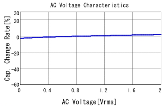
■ GCJ188R71H103KA01 C-AC Voltage capchange, DCOV, 25.0d
