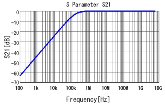
■ GCJ188R71H103KA01 S21 DC0V, 25degC
