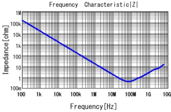
■ GCJ188R71H103KA01 |Z| DCOV, 25degC
